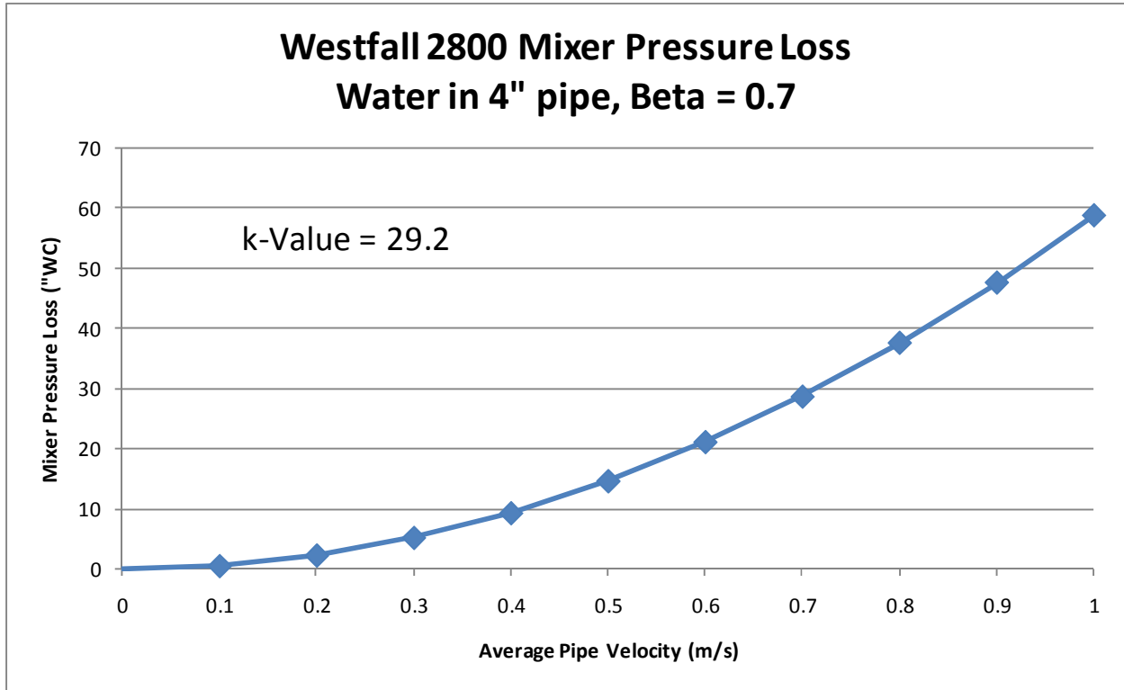
Figure 2: Pressure loss of mixer at various flow rates.
