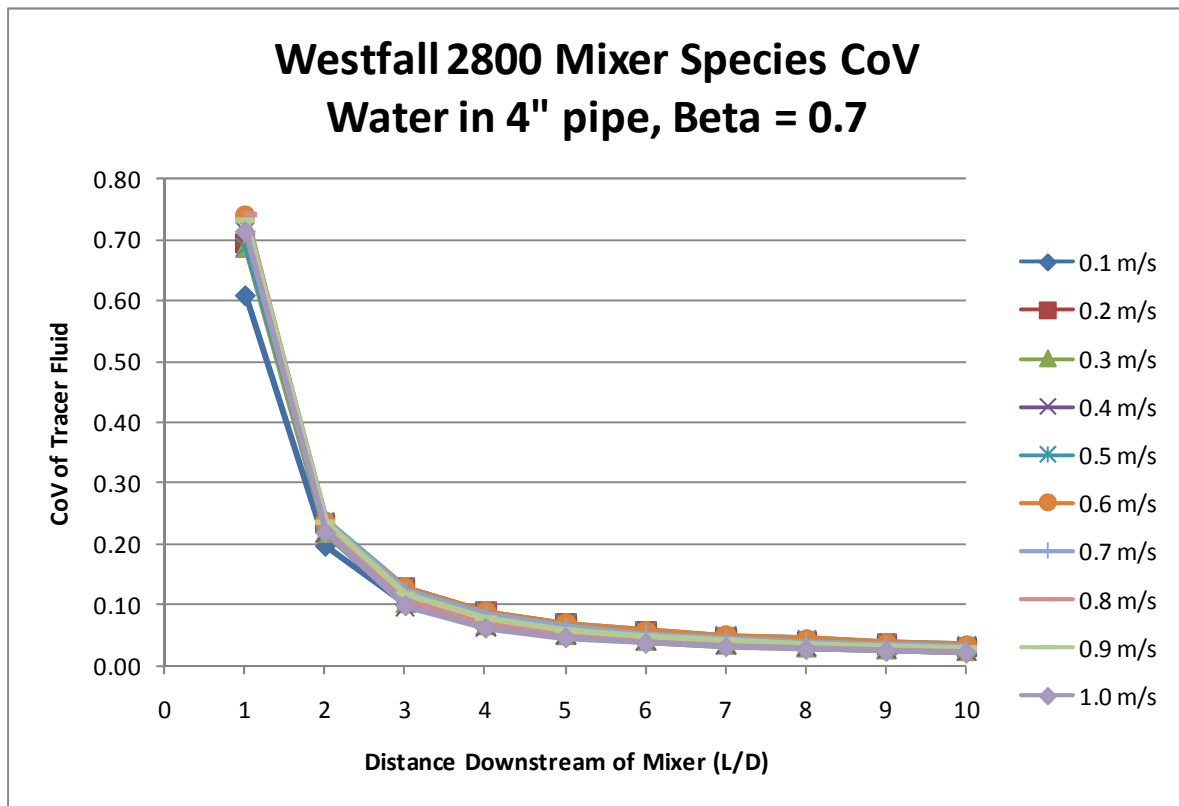
Figure 1: CoV of tracer fluid downstream of mixer.
