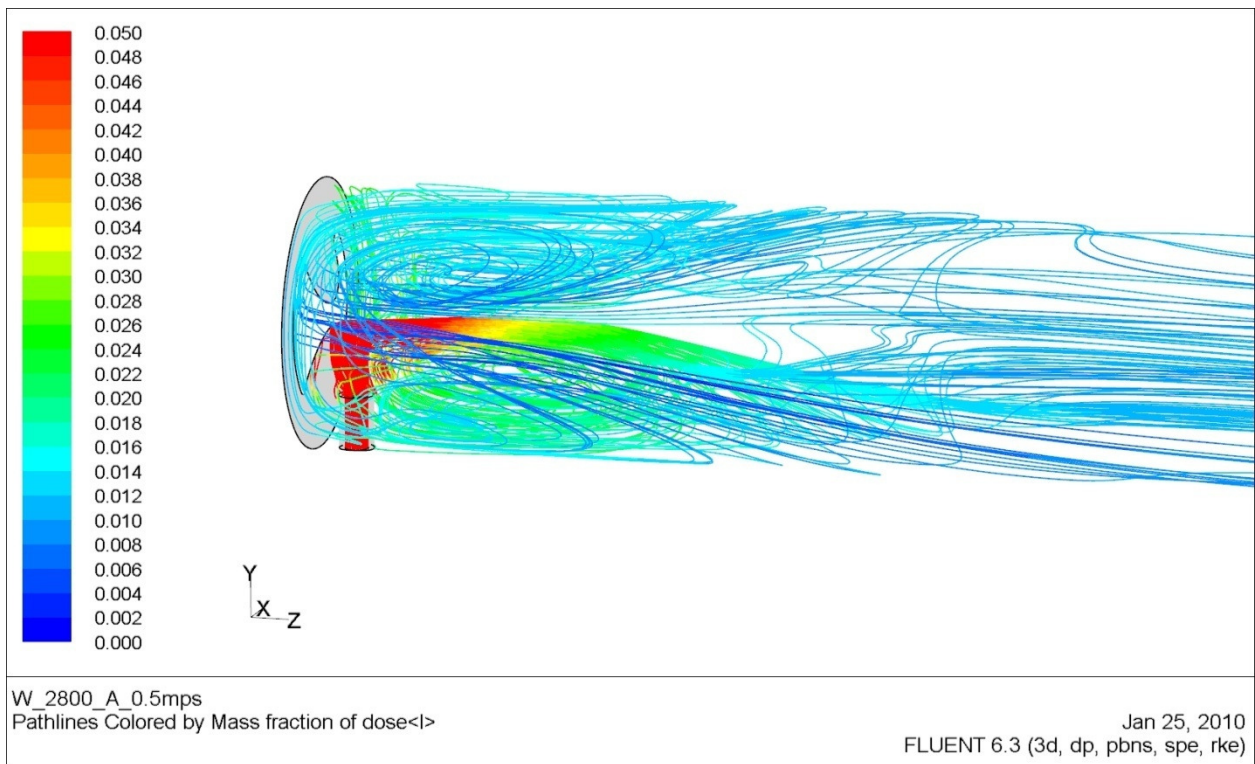
Figure 5: Pathlines released from the dosing port, colored by tracer mass fraction (average value = 0.01)
