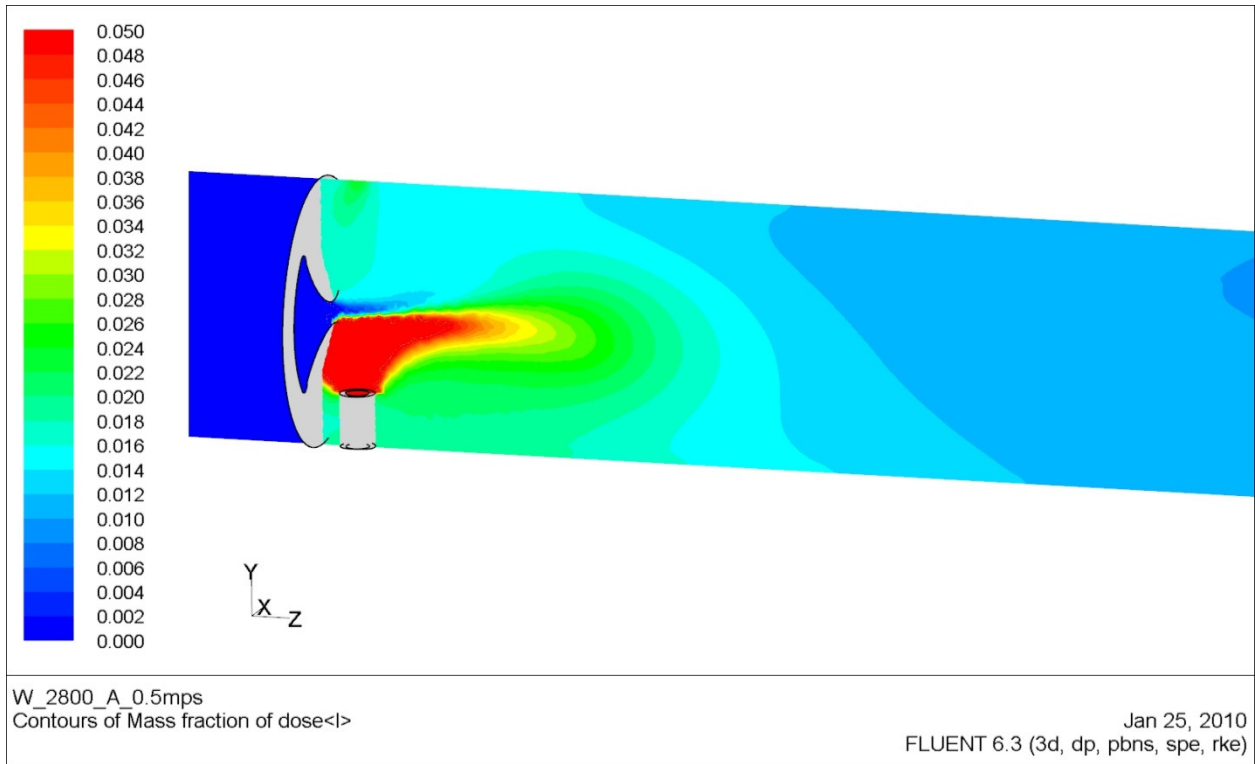
Figure 4: Contours of tracer fluid mass fraction (average value = 0.01)
