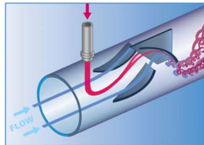
Westfall Model 6000 Counter-Swirl, Low Headloss Mixer
